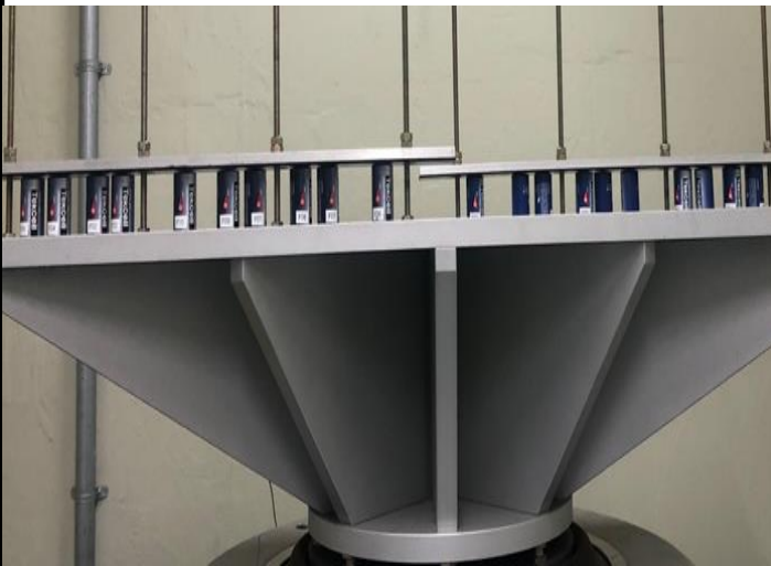
Photo.05 – Photographs of specimen before & after Vibration test (Undischarged cells)
